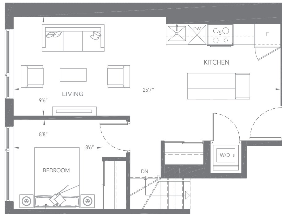
MAIN FLOOR
