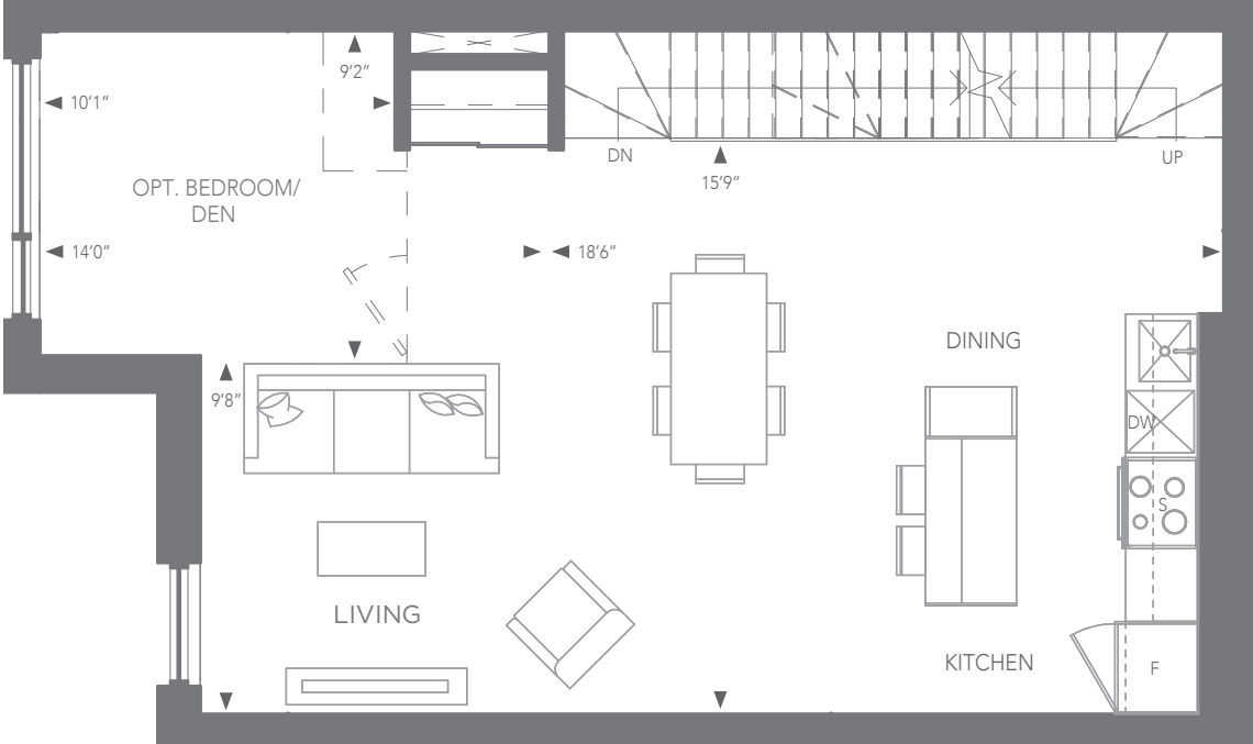
SECOND FLOOR
