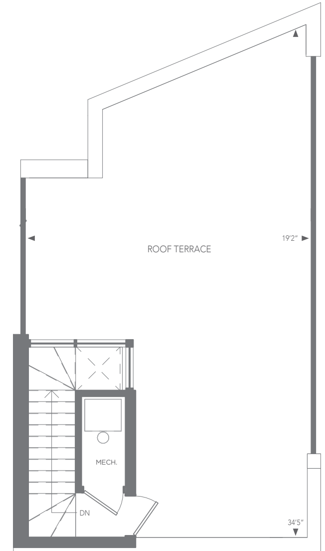
ROOF TERRACE
